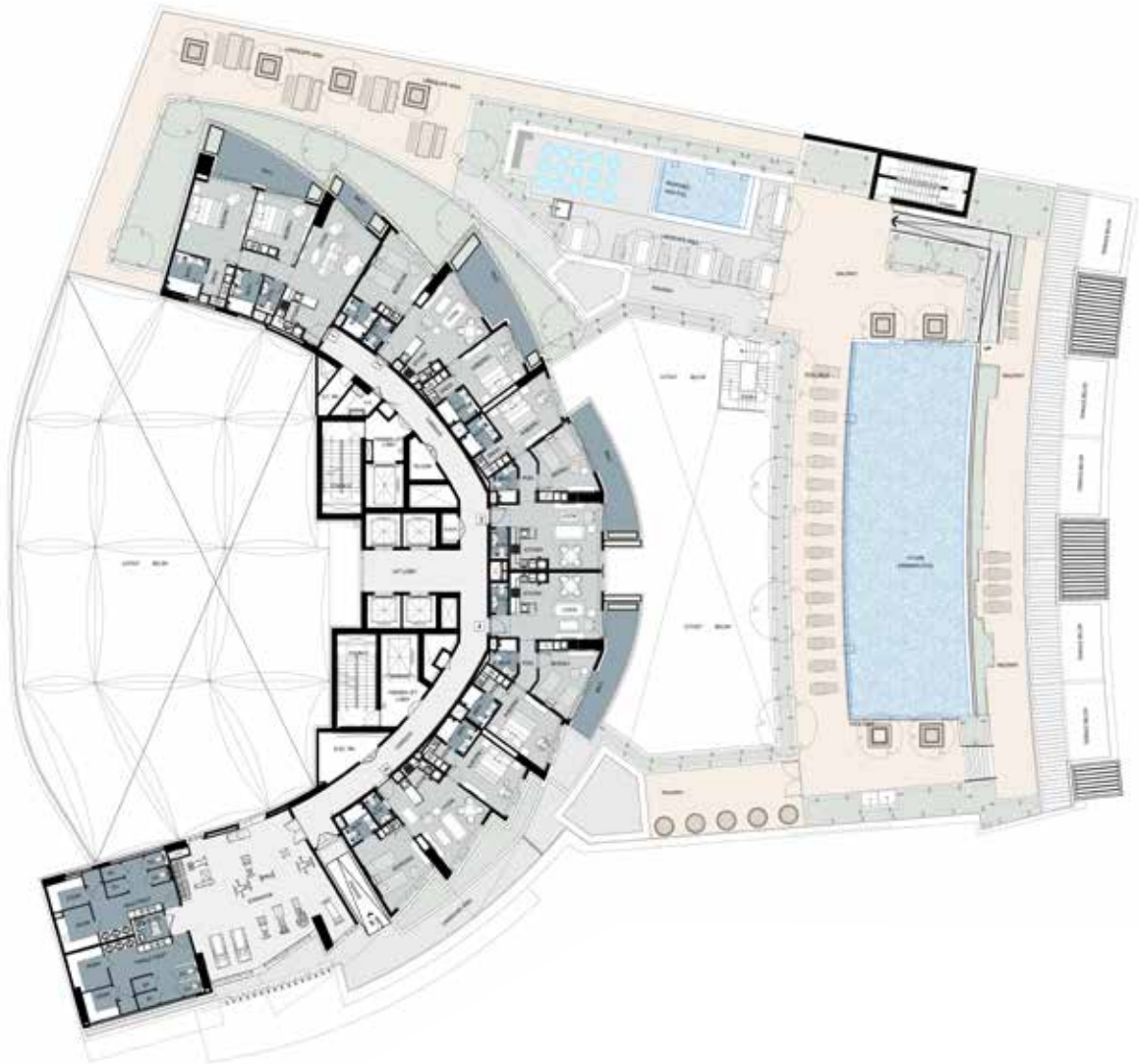
Level 1 Floor
