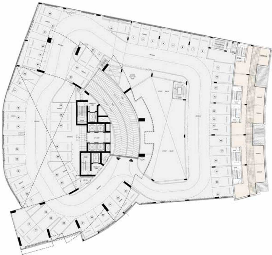
Level 2 Podium
